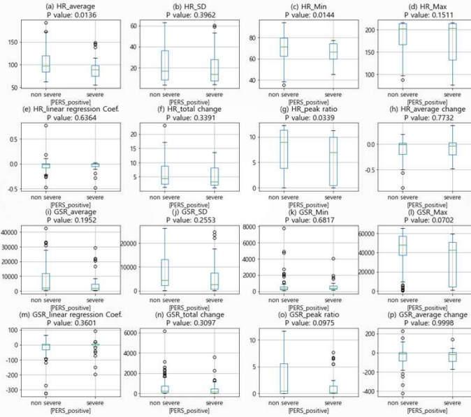
Boxplot grouped by PERS_positive
