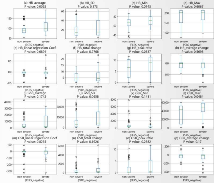
Boxplot grouped by PERS_negative
