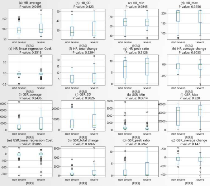
Boxplot grouped by PERS
