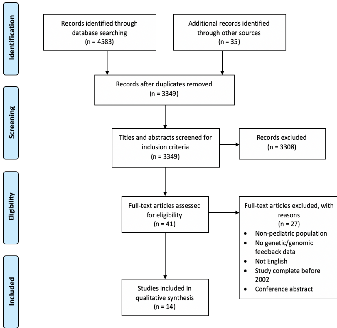
Figure 2. Prisma diagram
